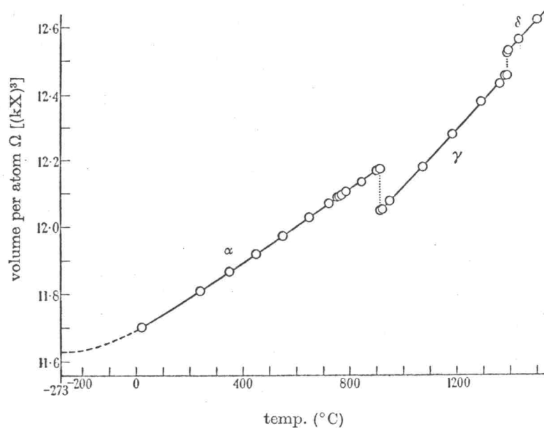
FIGURE 1c. Volumetric expansion of pure iron.
