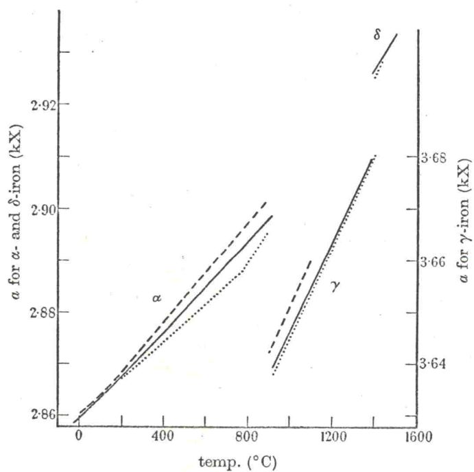
FIGURE 2. Variation of lattice parameter of pure iron with temperature. ----- Esser & Müller (1933); ..... Schmidt (1933); — Present results.
